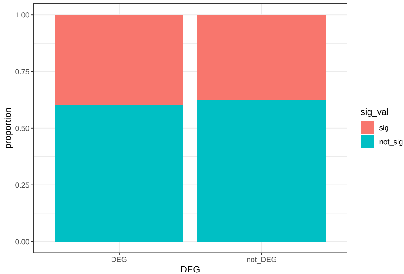
EPI DARs and not-DARs within 2kb of TSS of DEGs at 24 hours
